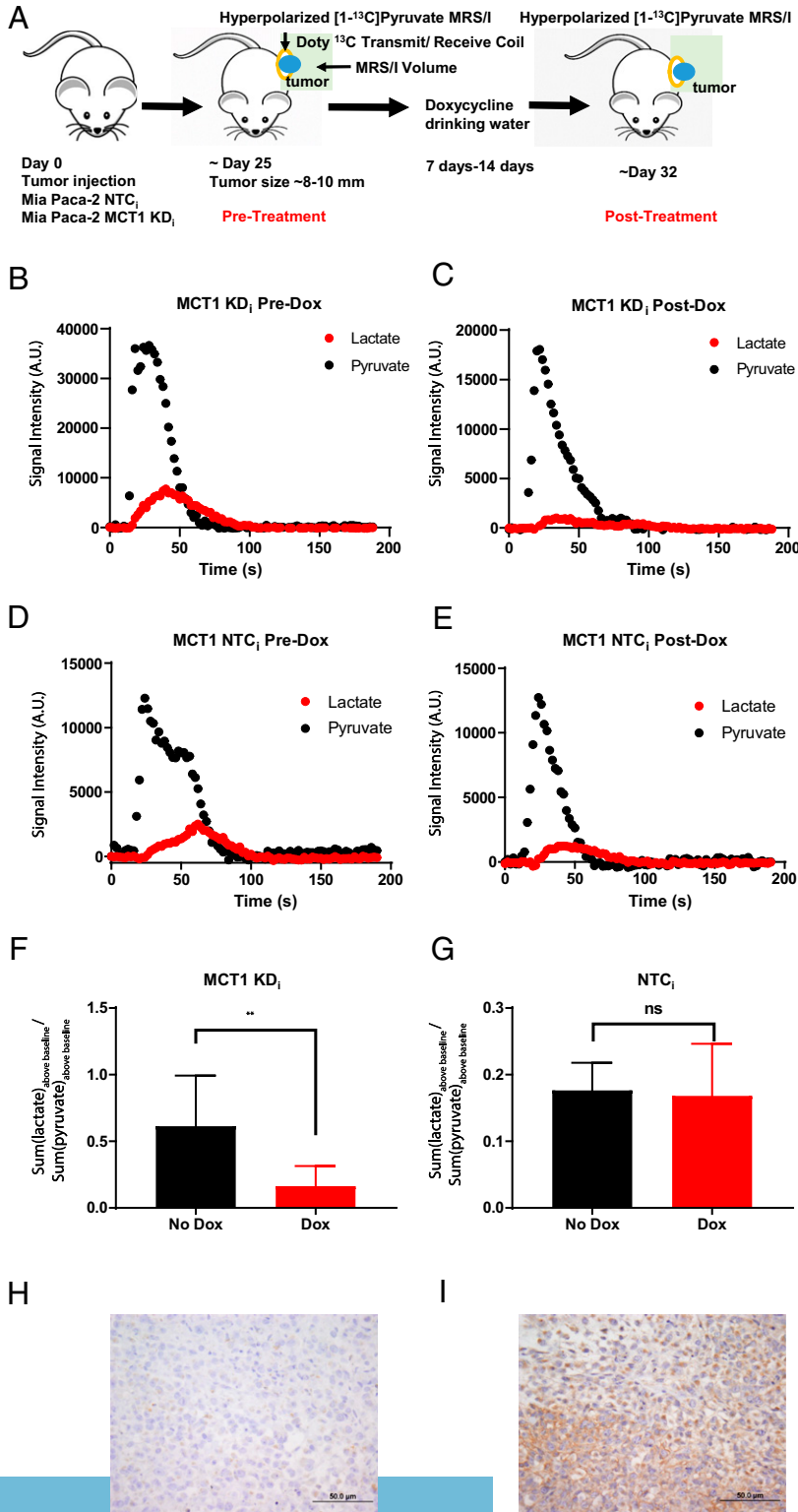
Fig. 4. Hyperpolarized [1- 13 C]pyruvate-to-[1- 13 C]lactate conversion in response to MCT1 expression in vivo. (A) Timeline of the animal study schedule. Each animal served as its own control pre- and postdoxycycline. (B and C) Hyperpolarized [1- 13 C]pyruvate and [1- 13 C]lactate spectra over time in a mouse bearing a Mia Paca-2 KD i tumor predoxycycline (B) and postdoxycycline (C) treatment. Hyperpolarized [1- 13 C]pyruvate and [1- 13 C]lactate spectra over time in a mouse bearing a Mia Paca-2 MCT1 NTC i tumor predoxycycline (D) and postdoxycycline (E) treatment. (F) The sum of hyperpolarized [1- 13 C]lactate normalized to the sum of hyperpolarized [1- 13 C]pyruvate of all mice bearing Mia Paca-2 MCT1 KD i tumors pre- and postdoxycycline treatment (n = 4 animals per group). (G) The sum of hyperpolarized [1- 13 C]lactate normalized to the sum of hyperpolarized [1- 13 C]pyruvate of all mice with Mia Paca-2 MCT1 NTC i tumors pre- and postdoxycycline treatment (n = 4 animals per group). Representative IHC staining for MCT1 from Mia Paca-2 xenograft tumors. All tumor sections were also stained with hematoxylin and eosin. (H) Mia Paca-2 MCT1 KD i tumors postdoxycycline treatment. (I) Mia Paca-2 MCT1 NTC i tumors postdoxycycline treatment. Error bars represent SD. **P < 0.01 (paired t test). A.U., arbitrary units; ns, not significant.
